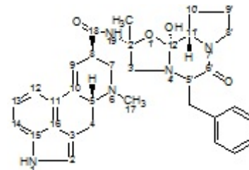
Ergotamine
