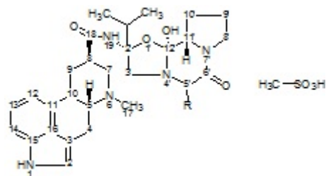
Ergoloid Mesylates
